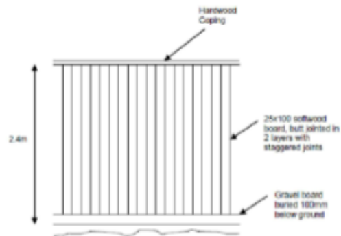
Acoustic Fence Elevation
