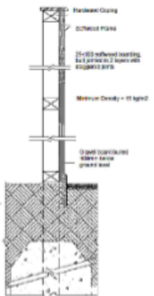
Acoustic Fence Cross Section
